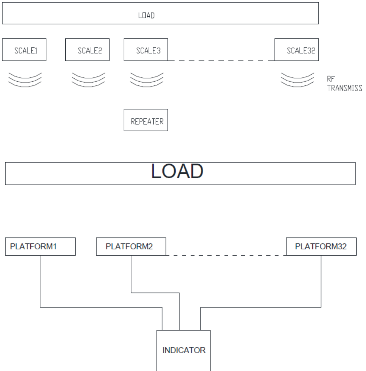
Figure 4 Examples of combined multi-platform weighing system
