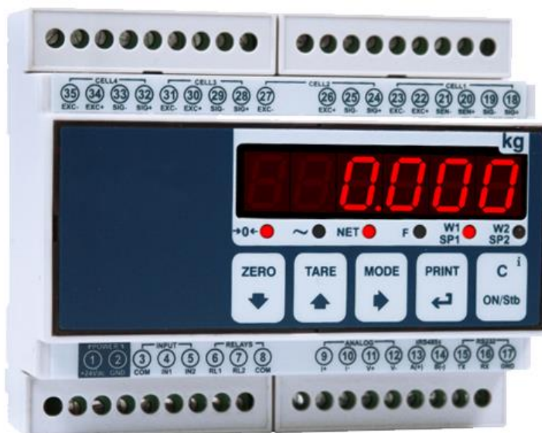
Figure 1 WA-03 family of indicators – enclosure example.
